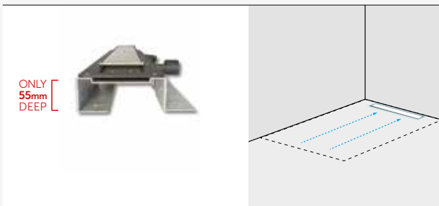
Linear Wall Drain - 1 way fall
