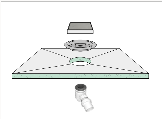
Quattro Grill, Trap and Drain
