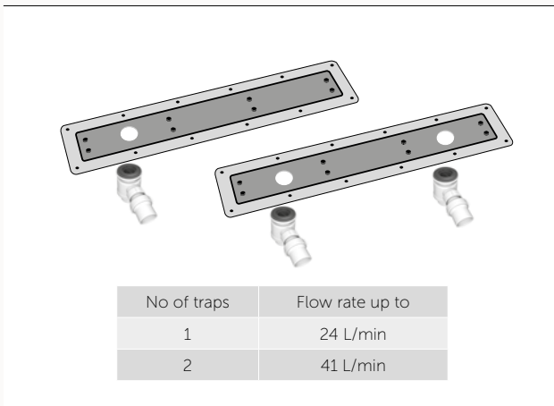
Drain and trap
