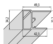
KUADRA 2.0 H 200 cm Deeper wall profile (+15 mm adjustability)
