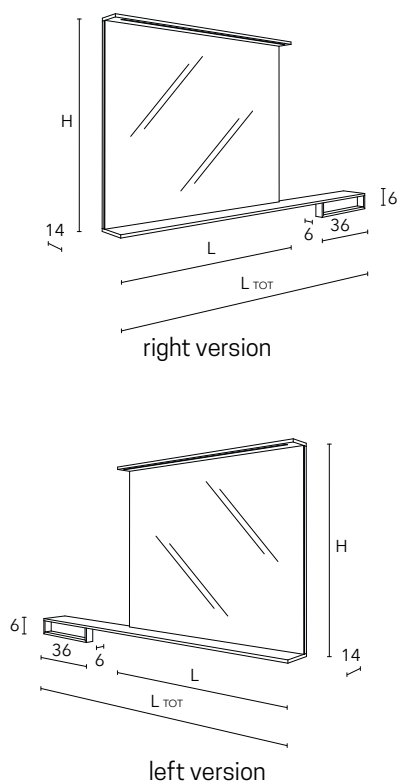
MIRRORS WITH ALUMINIUM SHELVES DEPTH 14 CM LED INTEGRATED IN UPPER SHELF AND LOWER SHELF 60 CM LENGTH WITH TOWEL RACK
