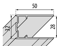
YOUNG H 200 cm Deeper wall profile (+15 mm adjustability)
