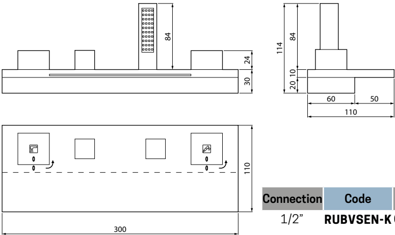
DECK MOUNTED BATH FILLER (for Style) with cartridge for progressive mixing, waterfall spout and shower design Marco Pellici
