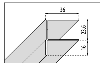
COMPENSATION +10 mm
