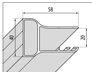
EXTENSION - FREE 1
