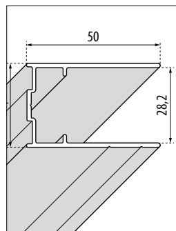
EXTENSION - FREE 3 +15 mm adjustability
