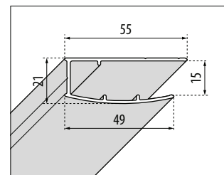
EXTENSION - FREE 2
