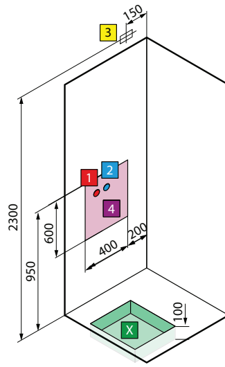
left version right version for model A100x80 - 2P120x80 - 2P120x90 - 2P120
